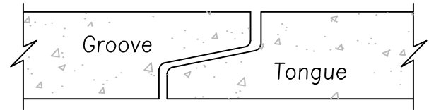
TYPICAL JOINT CROSS SECTION
